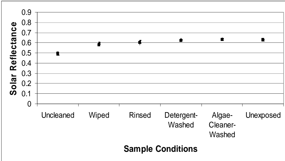
Figure 2: Solar Reflectance of Samples 9-10 and 14-15
