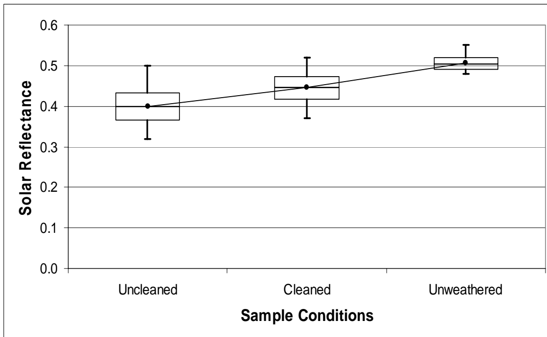
Figure 5: Solar Reflectance of Samples Analyzed at the NRC
