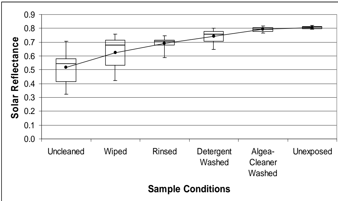
Figure 3: Solar Reflectance of Samples 1-8 and 11-13
