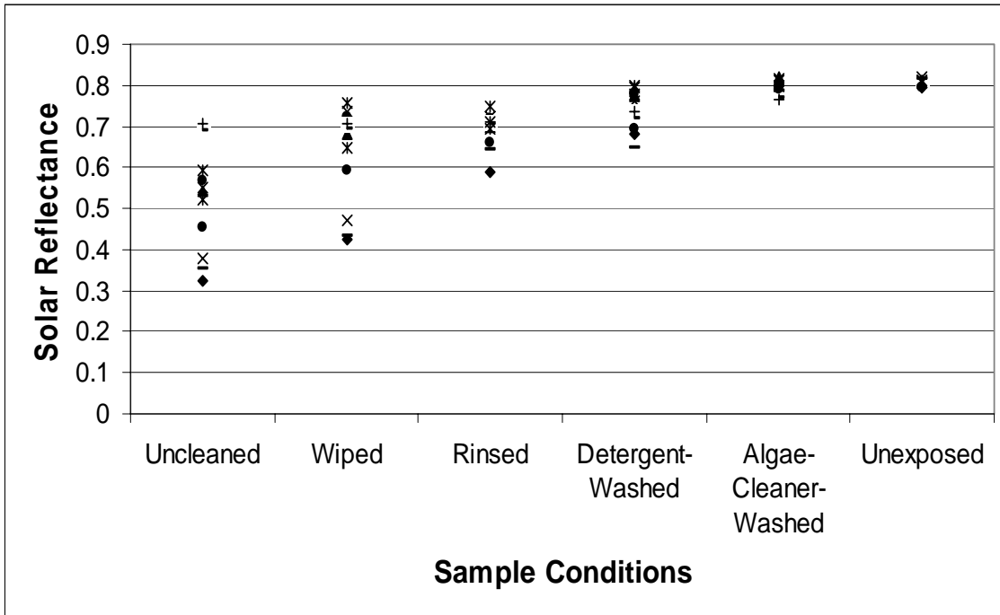
Figure 1: Solar Reflectance of Samples 1-8 and 11-13
